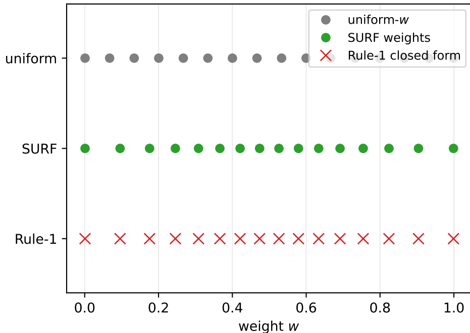
Steered weights (SURF \approx Rule-1)
