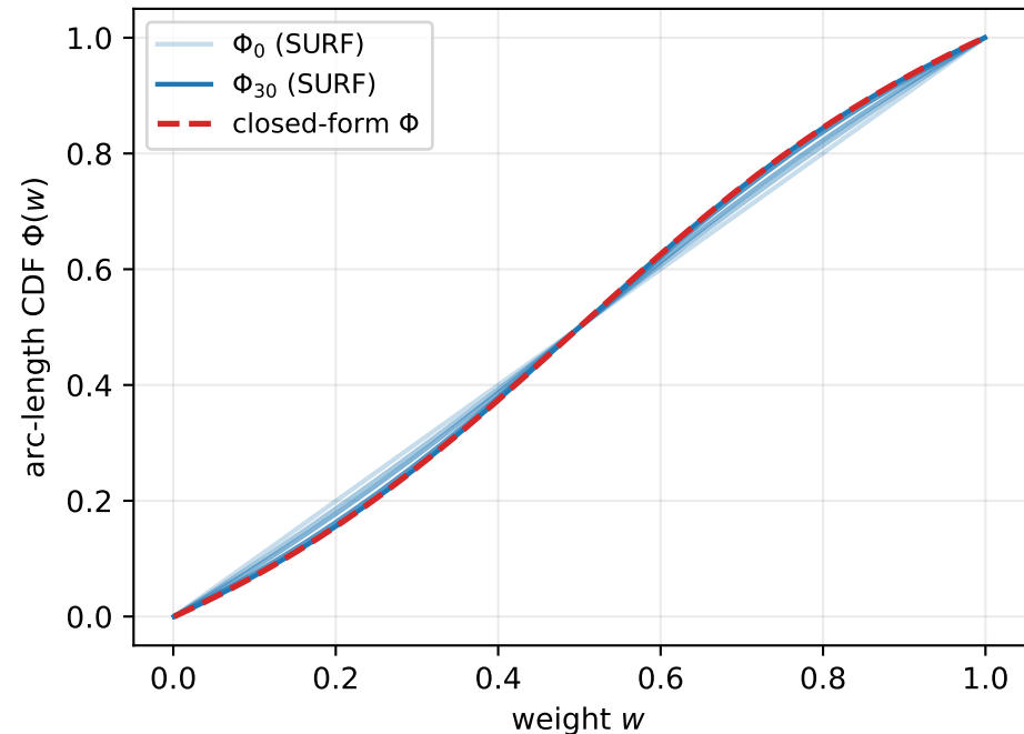
SURF CDF estimate \Phi_t converges to closed form
